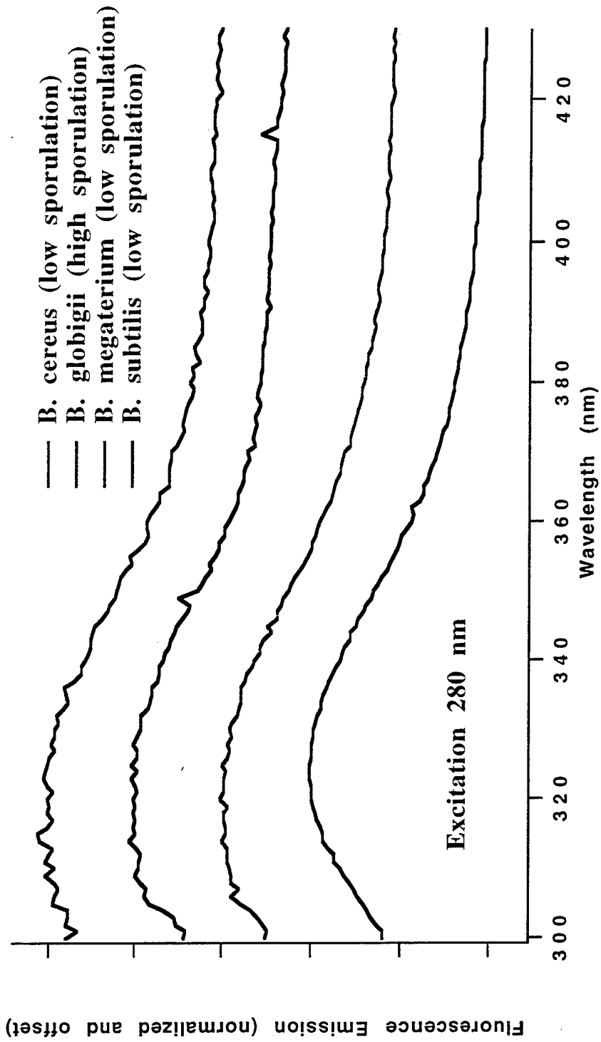
Figure 19. Fluorescence spectra of B. anthracis simulants suspended in water
