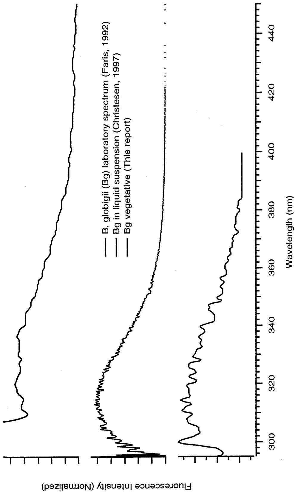
Figure 20. Comparison of fluorescence from this work and literature spectra
